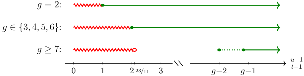
Figure 1: Visualization of the existence bounds obtained in FGH’25. Red zigzag lines indicate values of \frac{u-1}{t-1} for which (t, u) -stable menus are not guaranteed to exist. Green solid lines indicate values of \frac{u-1}{t-1} for which (t, u) -stable menus exist for all menu selection problems. Green dotted lines indicate that existence is only guaranteed for menu selection problems with complete preferences.
