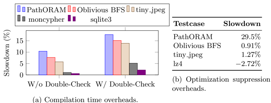
Fig. 1: Overheads from compilation process and optimization suppression.
