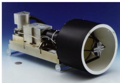
Figure A1: The Clementine LWIR sensor (Image from Shannon, "The Clementine Satellite").
