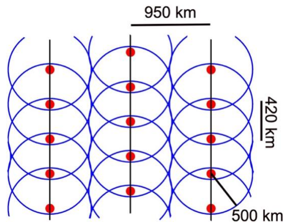
Figure 4. The alternate constellation. This constellation again has 2,000 satellites in 20 orbits (indicated by the vertical lines) with the same spacing between orbits as in Figure 3 (950 km at 25 degrees latitude). In this case the dots represent a single interceptor rather than a group of five as in Figure 3. The distance between the 100 interceptors within each orbit is 420 km for 300-km altitude orbits. For the interceptors to leave no gaps in coverage, each interceptor must be able to reach out in a circle of about 500 km radius during the time it has to fly to the target missile—compared to 950 km for the original constellation—as well as the distance of the intercept point above or below 300 km. In this constellation only a single interceptor could reach missiles passing through the areas where the circles do not overlap.
