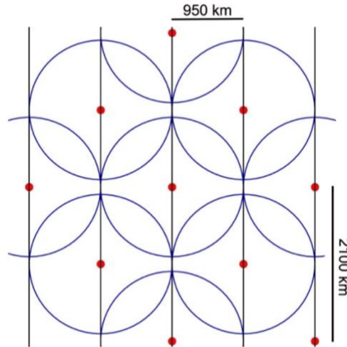
Figure 3. A version of the original Booz Allen Brilliant Swarms constellation shown in Figure 2, but with the circles showing the required coverage area of the interceptors to give complete defense coverage. The size of the circles is set so that there are no gaps in the coverage of the constellation. For 300-km altitude orbits the groups of interceptors are separated by 2,100 km along the orbit, and the spacing between orbits at 25 degrees latitude is 950 km. Each interceptor must be able to reach out in a circle of 950 km radius during the time it has to fly to intercept the missile, as well as the distance of the intercept point above or below 300 km.
