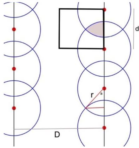
Figure D1: The dots represent interceptor satellites in the alternate constellation discussed in the text. The orbital planes are shown as vertical lines separated by a distance D , which depends on latitude. The interceptors are separated by a distance d . The circles of radius r represent the area around each interceptor that can be covered by that interceptor.
