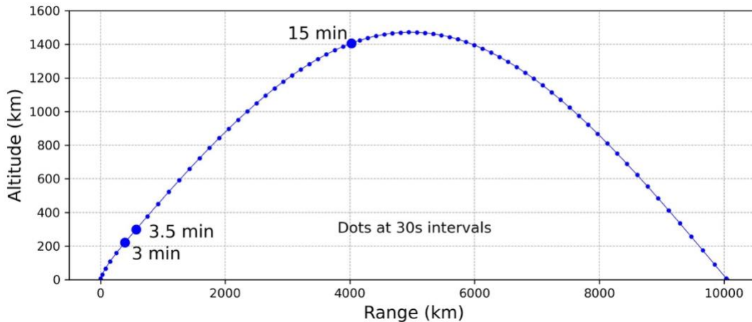
Figure 1. A standard trajectory for a 10,000 km-range missile. Booster burnout occurs at 3 minutes after launch and ascent phase is assumed to end by 3.5 minutes. The dots show the location at 30 second intervals.
