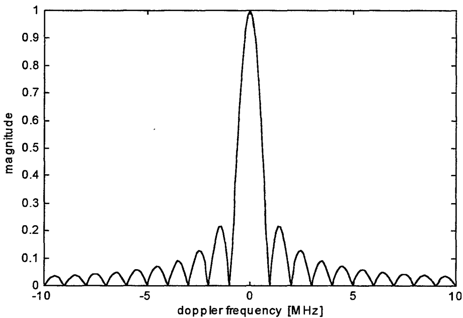
Figure A.5. Frequency profile of the ambiguity diagram of a single pulse. (pulse width =1 microsec)
