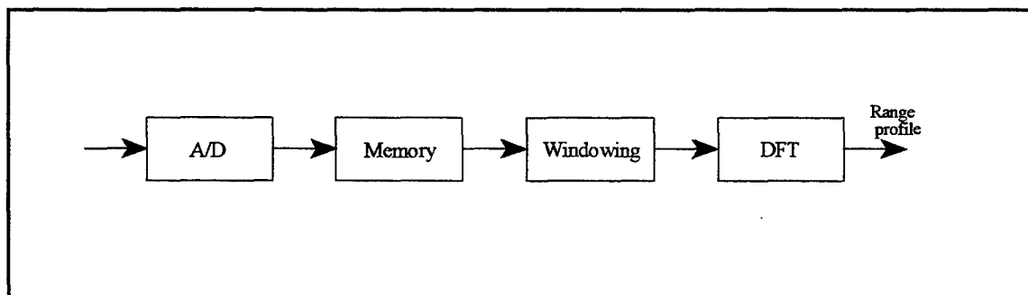
Figure 3. Elementary processing.
