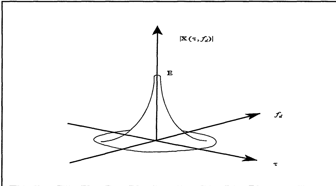
Figure A.1. An approximation to the ideal ambiguity diagram "After Ref. [1]."
