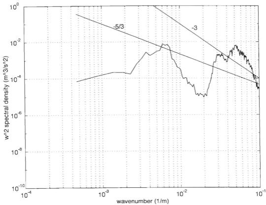
Figure 18. Windowed spectrum of w for Standard Depth 1. w 2 spectral density versus wavenumber.
