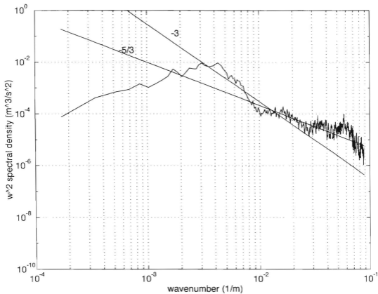
Figure 19. Windowed spectrum of w for Standard Depth 2. w^2 spectral density versus wavenumber.
