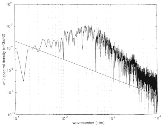
Figure 29. Spectrum of w for Standard Depth 4. w^2 spectral density versus wavenumber.
