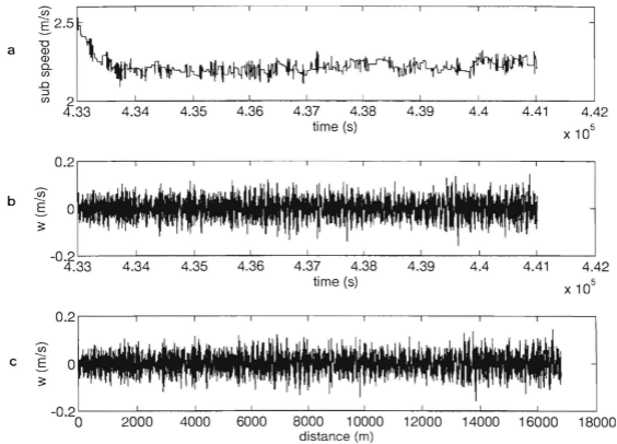
Figure 14. Standard Depth Case 1 for (a) submarine speed versus time, (b) vertical velocity ( w ) versus time and (c) vertical velocity versus distance.
