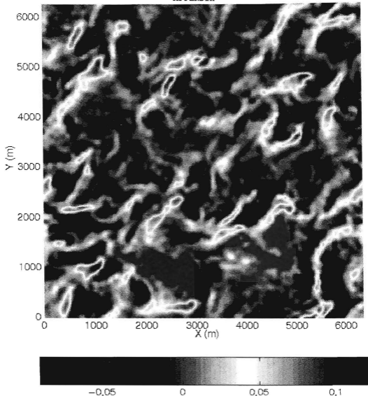
Figure 1. Vertical velocity as a function of X and Y, from the LES model at 125m depth at an instant in time.
