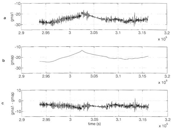
Figure 24. Standard Depth 2. (a) Observed gravity versus time. (b) Gravity anomaly versus time. (c) Observed gravity with gravity anomaly removed.
