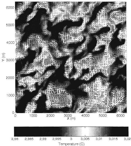
Figure 2. Same as Figure 1, except for temperature and horizontal velocity.
