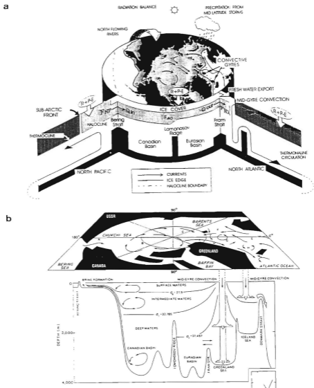
Figure 3. (a) Schematic of Arctic Ocean climate connections. Shaded ovals indicate the present sites of convection in the Greenland and Iceland Seas (from Aagaard and Carmack, 1994). (b) Schematic circulation and water mass structure in the Arctic Mediterranean (from Aagaard et al., 1985).
