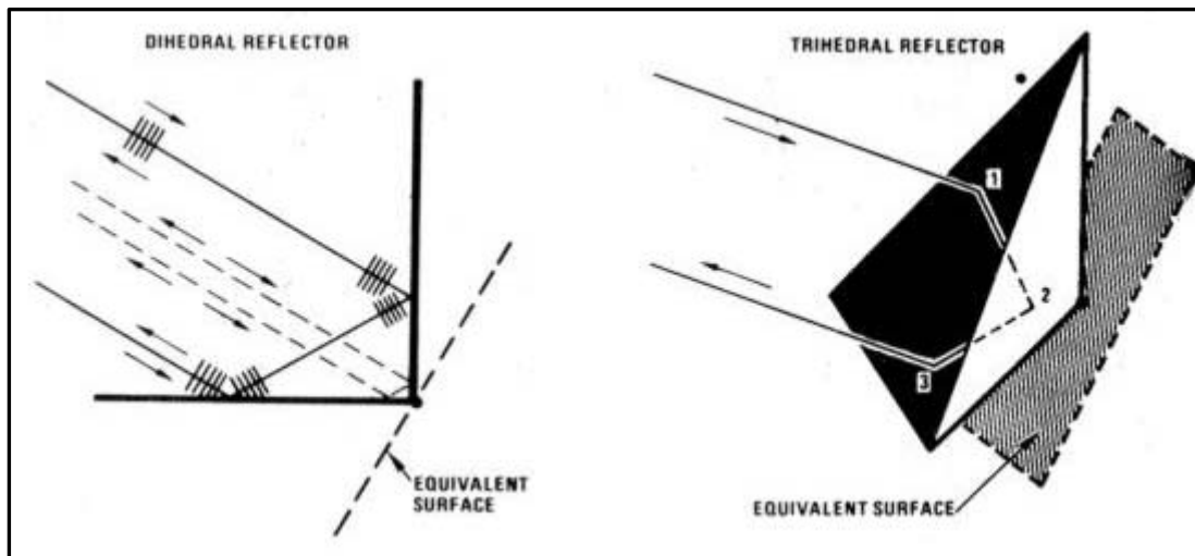
Figure 41. Corner Reflectors From [102]
