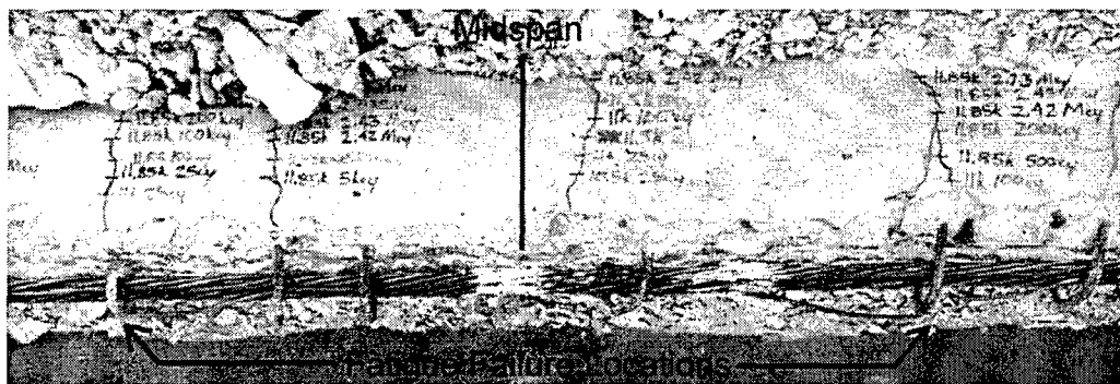
Figure 4-49 Photograph of Beam 3 After Removal of Concrete to Expose Strand
