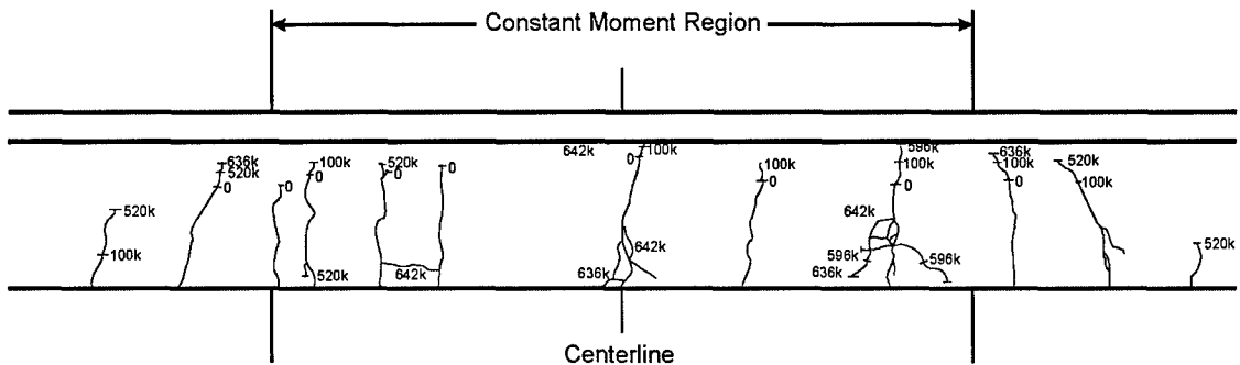
Figure 4-13 Observed Crack Pattern at End of Fatigue Tests—Beam 4
